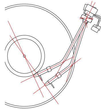
Figure 3.23: A correctly-designed and aligned pivoting tonearm has a tracking error of 0^\circ at only two locations on the disk.
