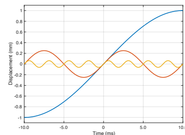
Figure 2.3: Three sine waves of different frequencies (from low to high: blue, red and orange curves), but with the same modulation velocity.
